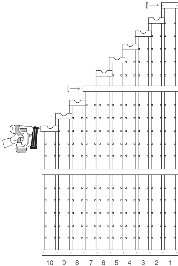
5 ATTACH THE TRIM PIECES
