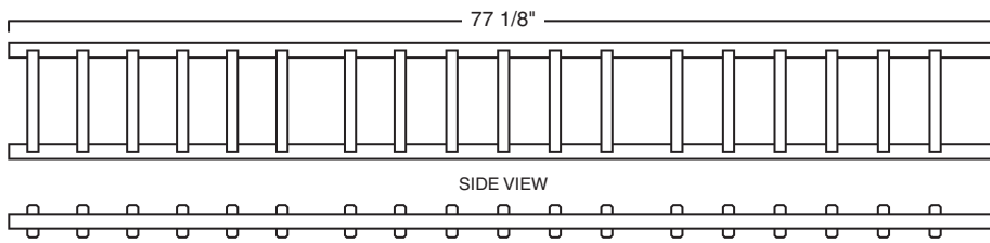
MIDDLE LADDER ASSEMBLIES (*VARIOUS LENGTHS) x 9
