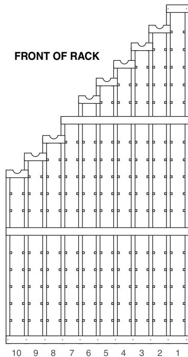
4 ATTACH THE 1-COLUMN CONNECTORS
